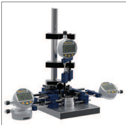
Bluetooth® indicators on a 4 points jig
