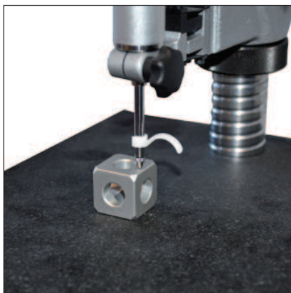
Lifting device on S_Dial PRO Basic
